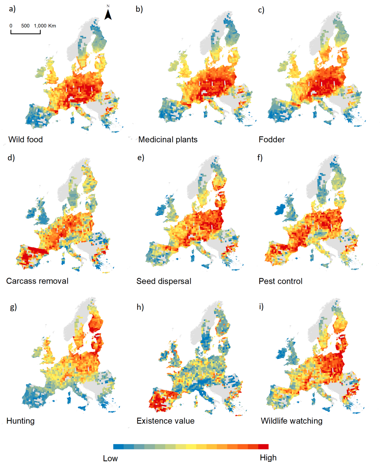
Fig. 1. Weighted provider richness for species-based services at 50 × 50 km resolution. The color categories display quantiles.
